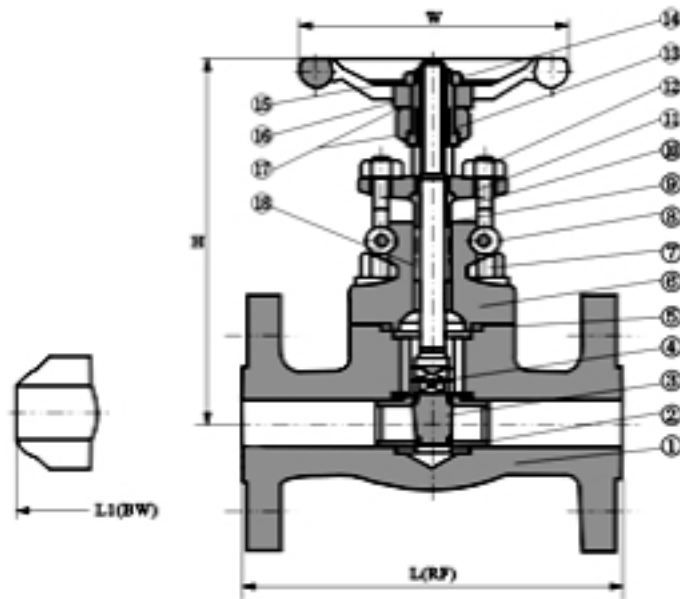
Forged steel flange gate valve 900Lb~1500Lb Material List
